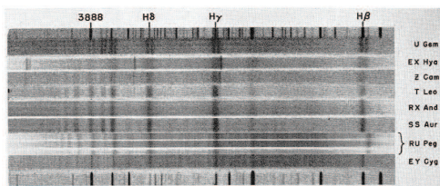
Fig. 1. Trailing spectra of Cataclysmic Variables by Kraft (1962).
